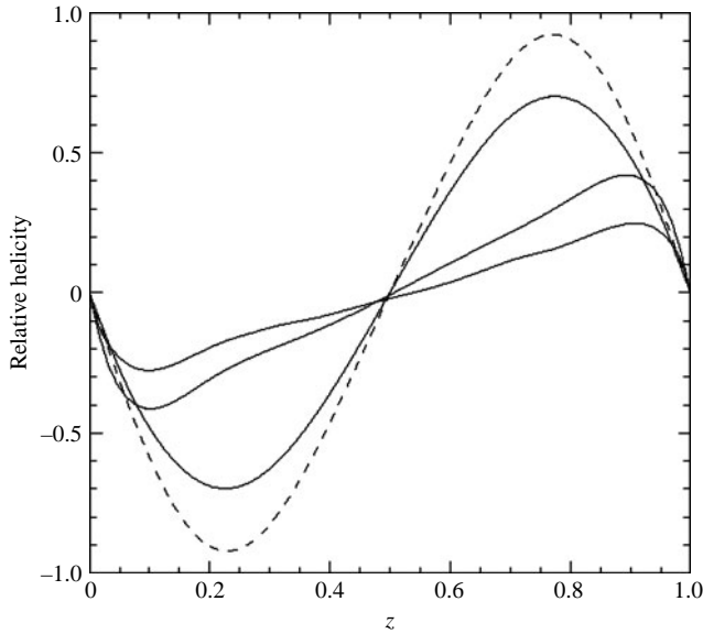
FIGURE 2. Snapshots of h(z) (the horizontally averaged relative flow helicity). The solid curves correspond to cases with \lambda=5 and Ra=80\,000 , 150\,000 and 500\,000 ; the helicity decreases with increasing Ra . The dashed curve corresponds to the case with \lambda=0.5 and Ra=80\,000 .
